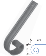
Ref. ↓ ↑ ↕ ↔ ↘ ↙ 03164 370 x 170 40x8
